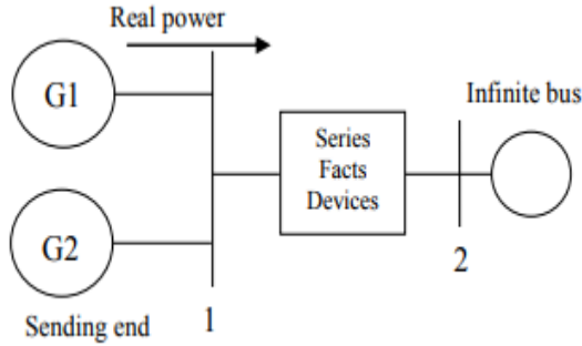
Figure 4. Test system with series FACTS device
