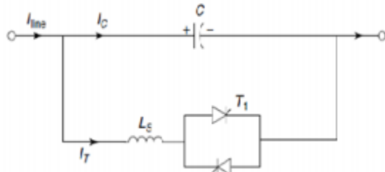
Figure1-Configuration of TCSC
