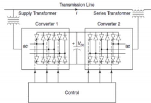
Figure3-Configuration of UPFC
