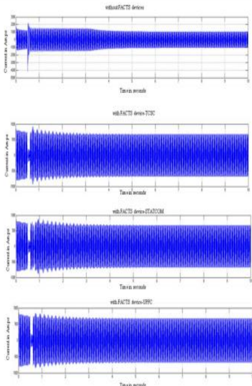
Figure 12. Simulation Result for Generator Current (I g )
