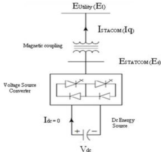
Figure 2-Configuration of STATCOM
