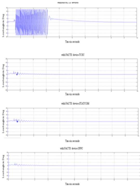
Figure 13. Simulation Result for Generator Load Angle ( \delta )
