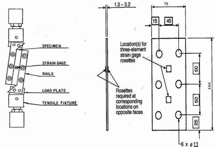
Fig: Two Rail Shear Test Method
