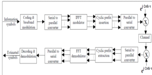
Fig.1: OFDM System
