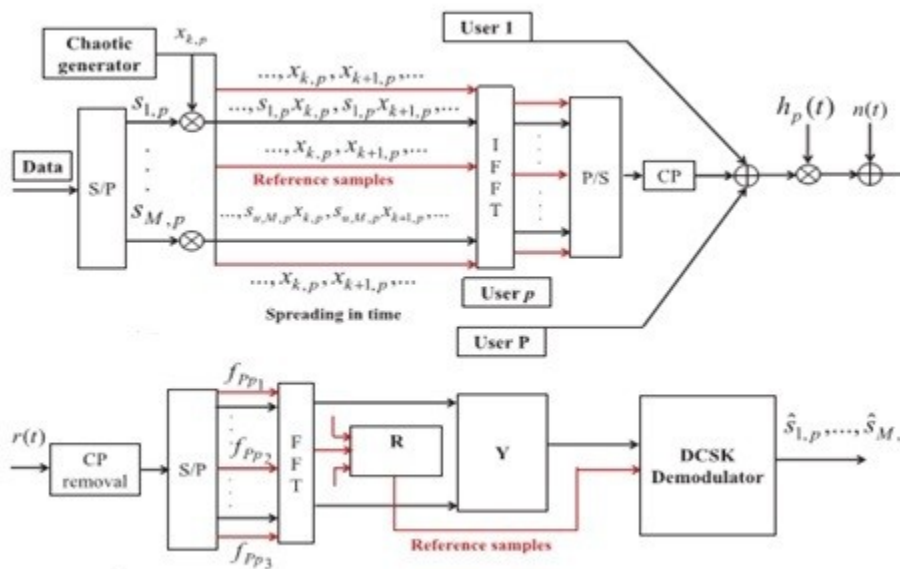
Fig.1 Block diagram of the MU OFDM-DCSK system consist of transmitter and receiver
