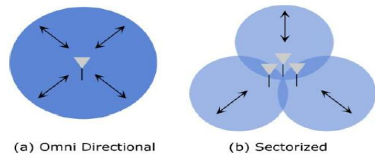
Figure 1: Non-smart antenna systems
