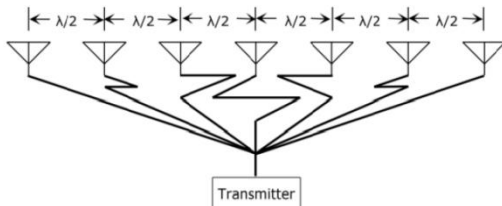
Figure 3: 7-Element 3\lambda Linear Array
