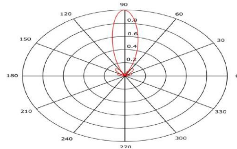
Figure 2: Three Wavelength Circular Aperture - Field Strength vs. Direction
