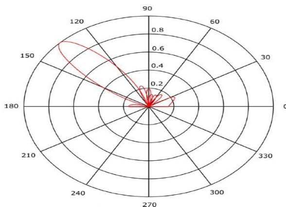
Figure 4: 3.5 Wavelength 8 Element Linear Array, Progressive 0.7\pi Phase Shift
