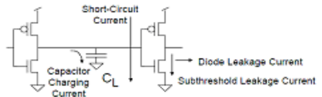
Fig.2 CMOS-Power-Dispersal
