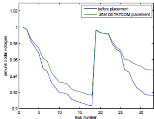
Fig.4. Voltage profiles for IEEE 33-bus system
