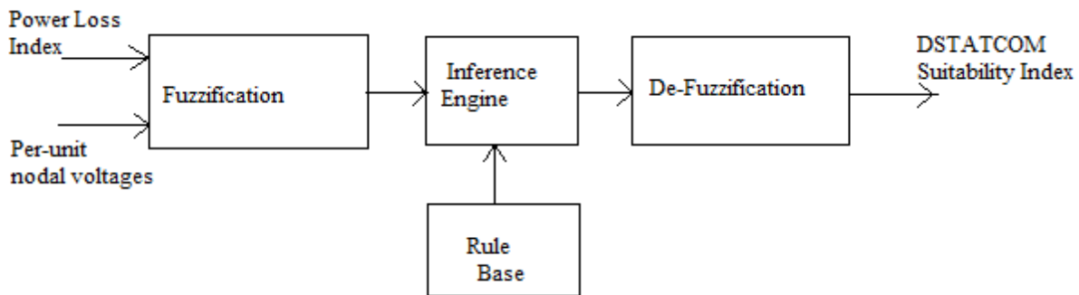
fig.3. Block diagram of Fuzzy inference system
