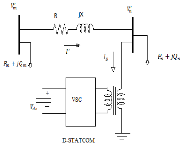
Fig.2. single line diagram of two bus distribution system with DSTATCOM
