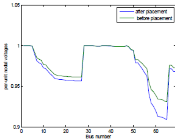
Fig.5. Voltage profiles for IEEE 69 -bus system
