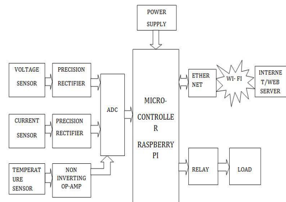
Fig2: Client block diagram
