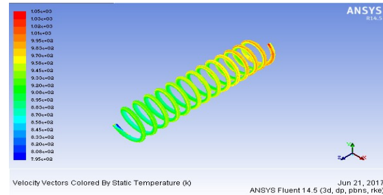
Fig 3.1velocity vectors colored by static temperature
