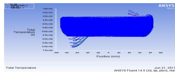
Fig 3.3 Graph of total temperature
