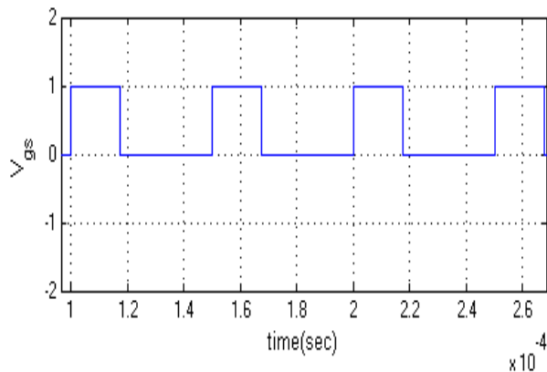
Fig.8 voltage ( V_{gs} )
