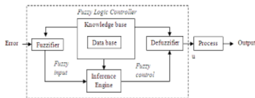
Fig 9. Structure of Fuzzy Logic Controller
