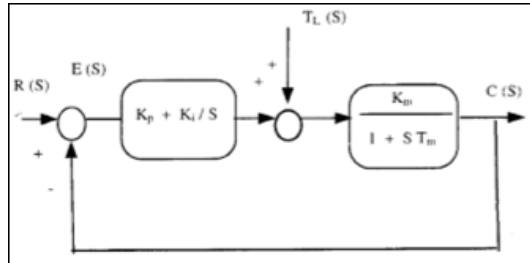
Fig.1 blok diagram with P-I controller
