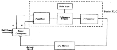
Fig.3 basic function of fuzzy logic controller
