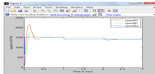
Fig 14. Comparative Speed scope
