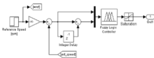
Fig 10. Block Diagram of FLC
