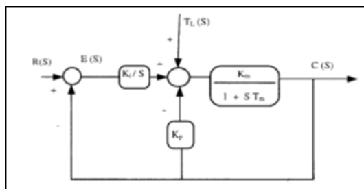
Fig.2 blok diagram with I-P controller
