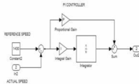
Fig 6. Basic model of P-I controller
