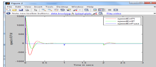
Fig 13. Comparative Speed Error Scope
