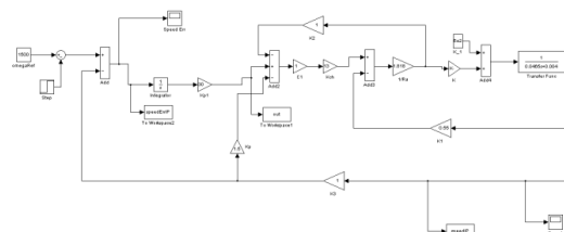
Fig 9. I-P controller
