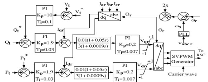
Fig. 2. RSC Controller
