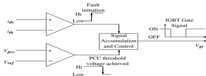
Fig. 5. BFCL controller
