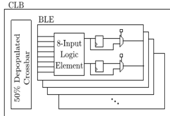
Fig.6. Hybrid CLB with a 50% depopulated intra-CLB crossbar depicting BLE internals for a fracturable (two optional registers and two outputs) architecture.
