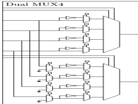
Fig.4. Dual MUX4 LE that utilizes dedicated select inputs and shared data Inputs
