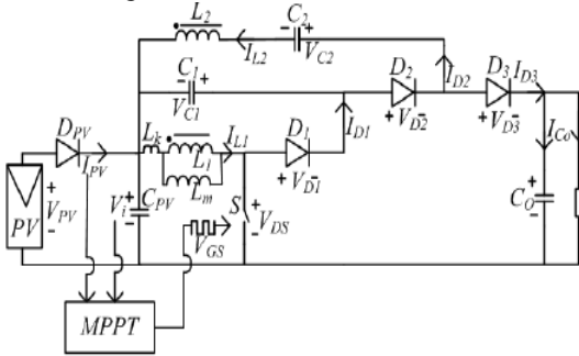
Fig. 3 Circuit diagram of proposed dc-dc converter
