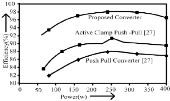
Fig.11. Efficiency versus load curve for the proposed dc-dc converter and comparison with existing versions;
