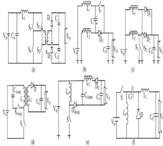
Fig. 2 Circuit diagrams of the high voltage gain dc-dc converters: (a) Isolated current-fed boost converter (b) Coupled inductor boost converter (c) Interleaved coupled inductor boost converter (d) Active clamp converter (e) Passive clamp converter (f) Intermediate Energy storage capacitor based converter
