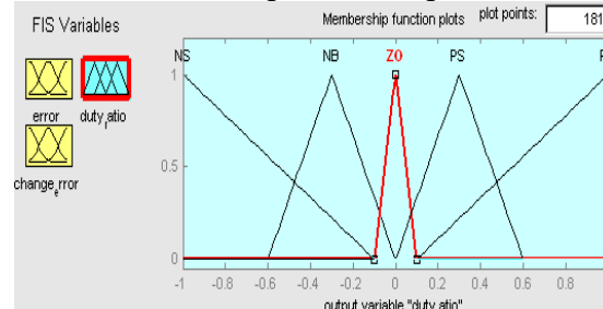
The Membership Function plots of duty ratio
