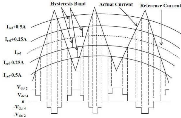
Fig.5: Hysteresis current control scheme for five level MLI-DSTATCOM
