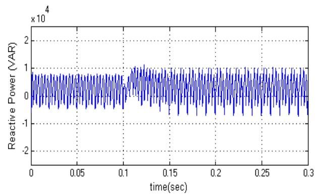
Fig.17 Output waveform of reactive power at supply side
