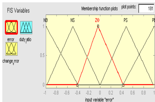
The Membership Function plots of error
