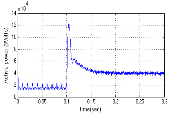
Fig.13 Output waveform of Active power at supply side
