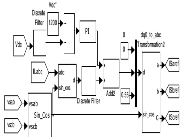
Fig.4 Shunt Controller using SRF
