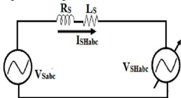
Fig.1 Block diagram of DSTATCOM
