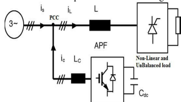
Fig.1 Block diagram of DSTATCOM
