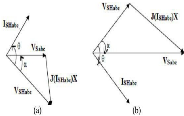
Fig.3 Phasor representation of DSTATCOM From the phasor diagrams it is clear that, DSTATCOM either generates or absorbs the reactive power by controlling the phase angle ( \alpha ) between V_{SHabc} and V_{Sabc} thereby regulating the magnitude of the V_{SHabc} and thus DC Link capacitor voltage.
