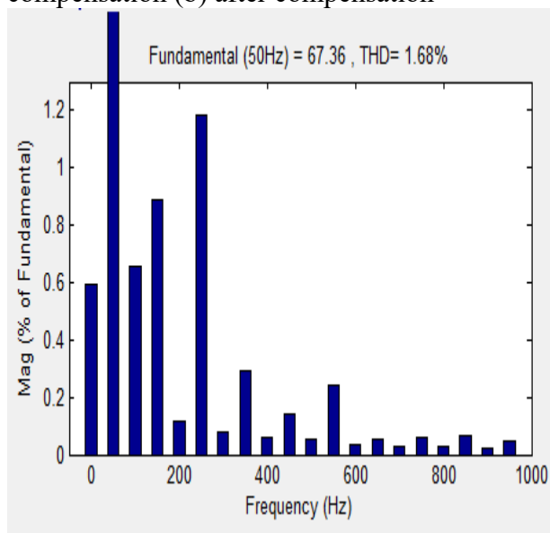
Fig.20 THD of Source current with fuzzy
