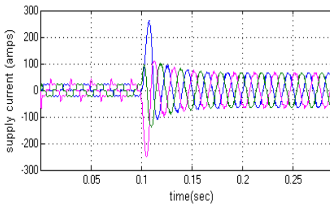
Fig.10 Output waveform of Supply current
