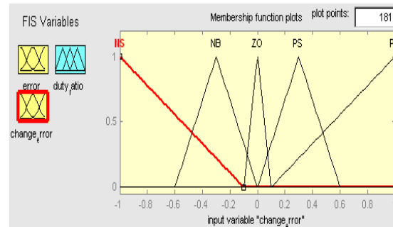
The Membership Function plots of change error
