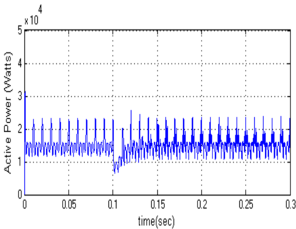
Fig.14 Output waveform of Active power at load side
