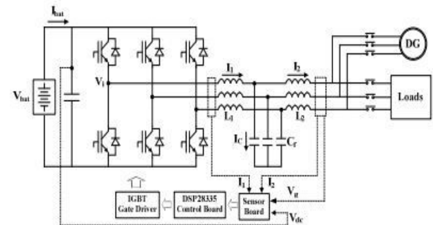
Fig.1 The configuration of a stand-alone microgrid
