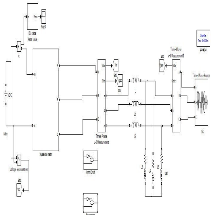
Fig.10 MATLAB and Simulink circuit for Proposed BESS
