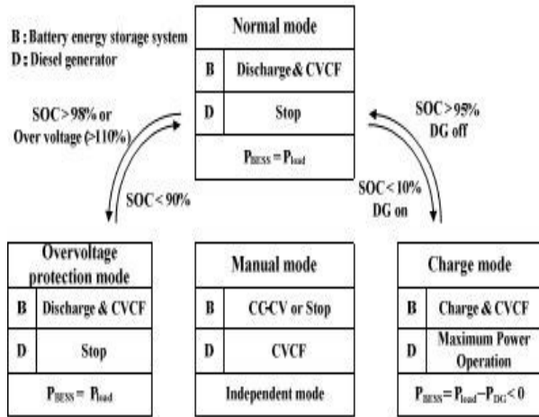
Fig.2: The operation mode of the stand-alone microgrid
