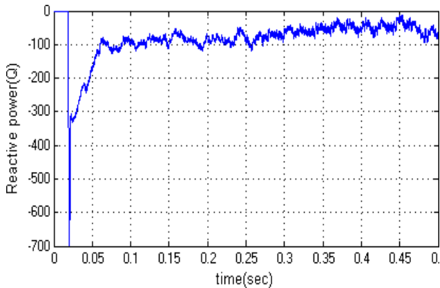
(b) BESS 40kW charging
