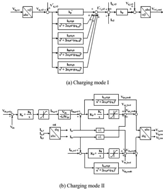
Figure3: Control of two charging methods Fig 3 shows control methods of the two charging modes in the stand-alone microgrid.
