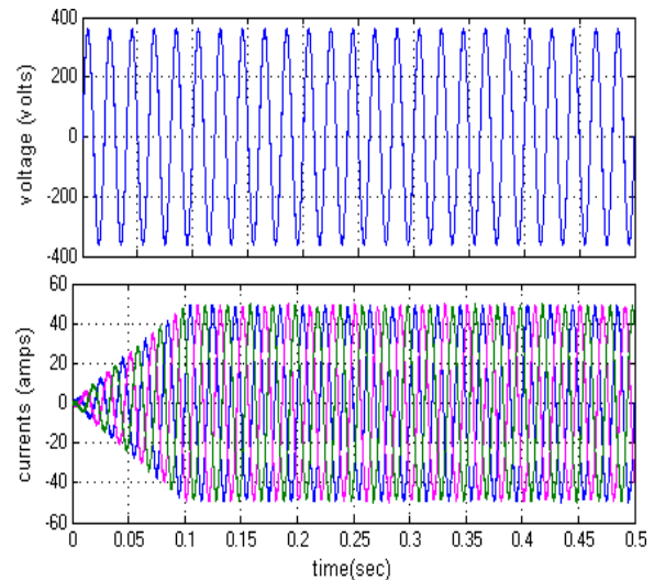
(a) BESS 40kW charging
