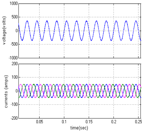
(a) Voltage and currents in 40kW
