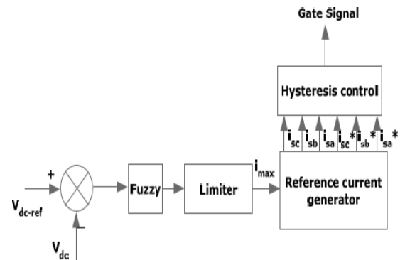
Fig.8. Conventional fuzzy controller
