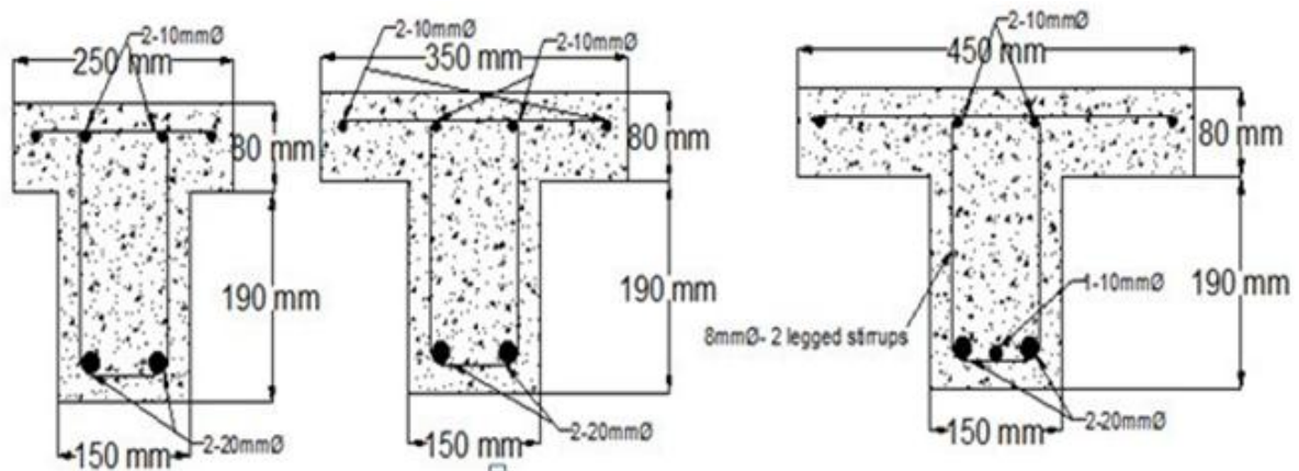
Figure-1 crosssection and reinforcement
