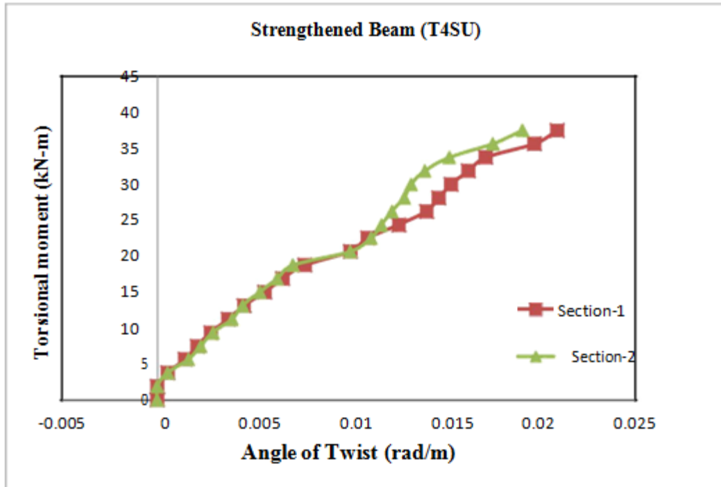
Figure-3 (A),(B),(C),(D),(E),(F) Are Curves Between Torsional Moment VS. Angle Of Twist
