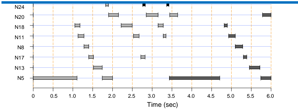
Figure 6: Transmission time-line for an ExOR transfer from N5 to N24. Nodes higher on the Y axis have lower ETX metrics to N24. The light gray bars show the transmissions in the first batch. The darker gray bars show part of the second batch.
