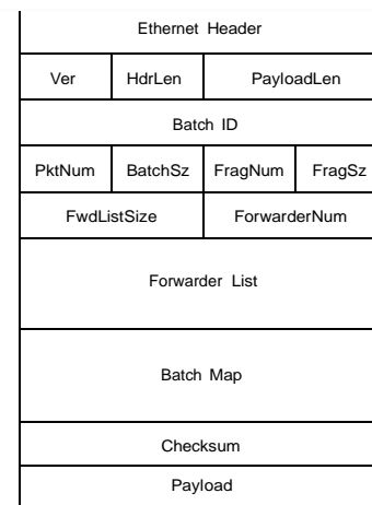
Figure 3: ExOR packet header format.
