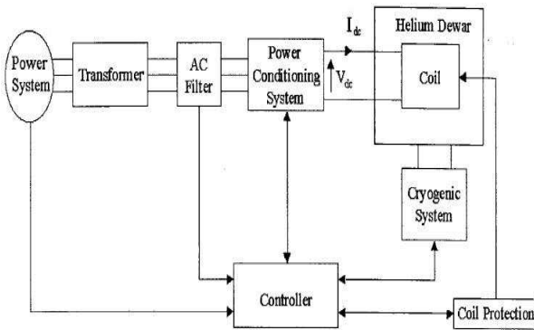
Fig. 1. Structure of SMES
