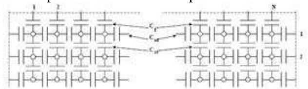
Fig. 4. Capacitive parameters in the entire coil
