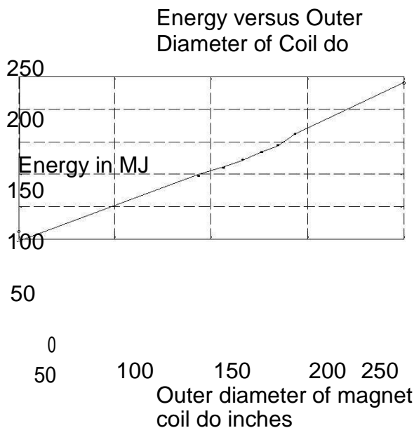
Fig .7. E-do curve of the SMES coil.
