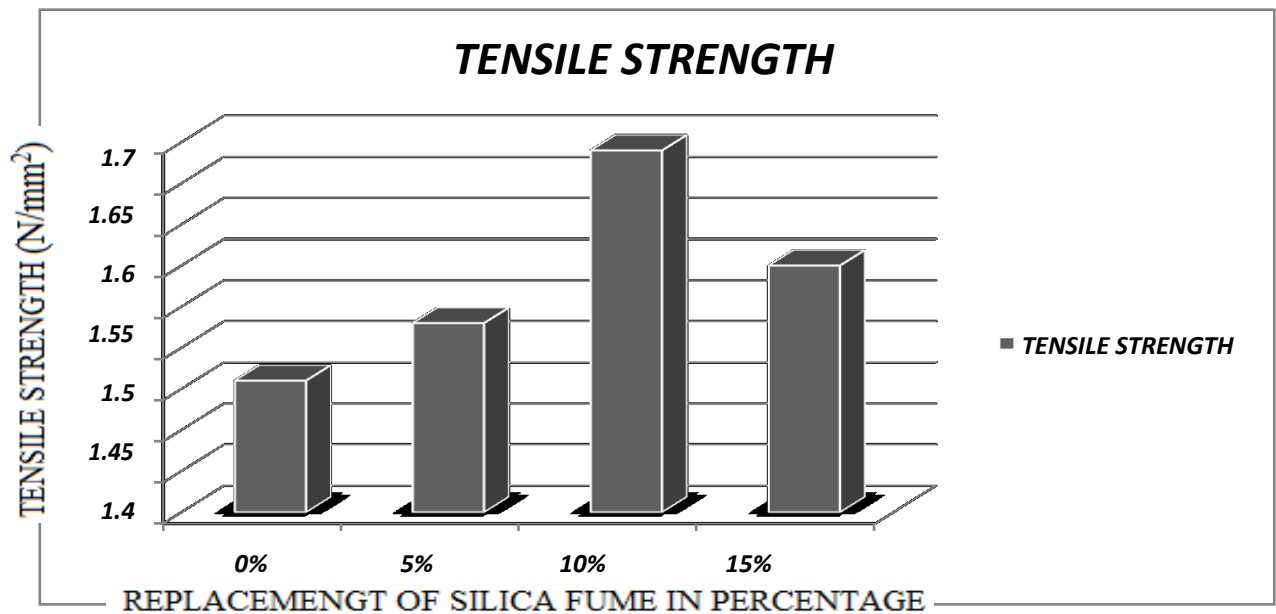
Fig2: Tensile Strength v/s % of Silica Fume
