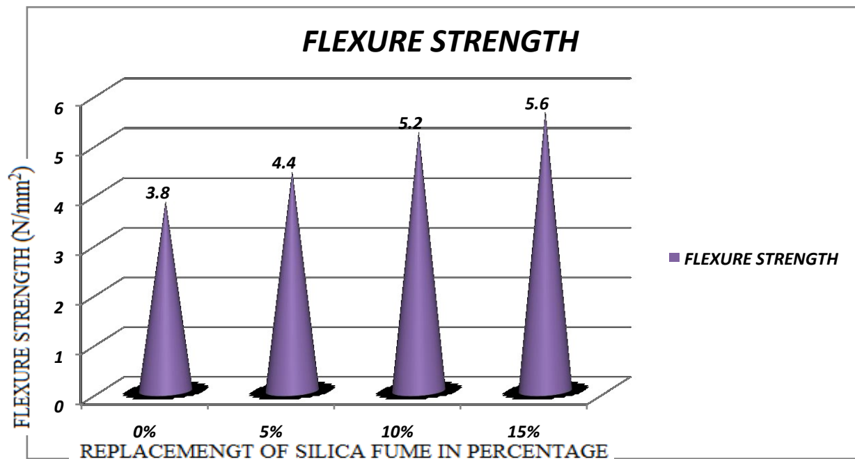
Fig 1: Flexural Strength v/s % of Silica Fume
