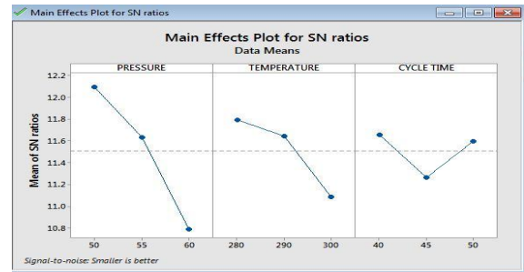
S/N ratio
