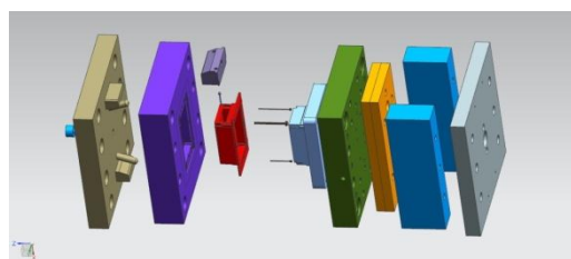
Exploded view
