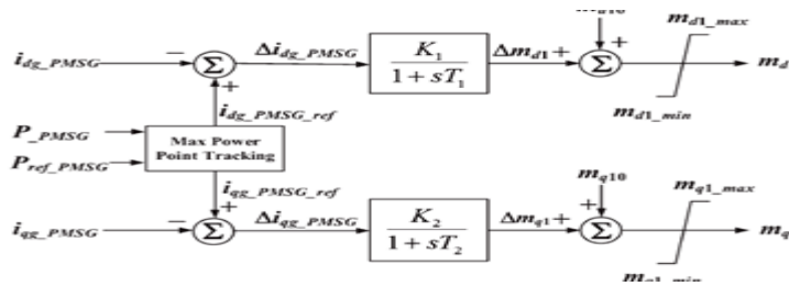
Fig-6: Control block diagram of the modulation indices of the VSC of the studied PMSG.
