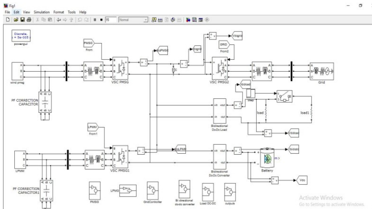
Fig 8. MATLAB/SIMULATION diagram of proposed wind and wave system
