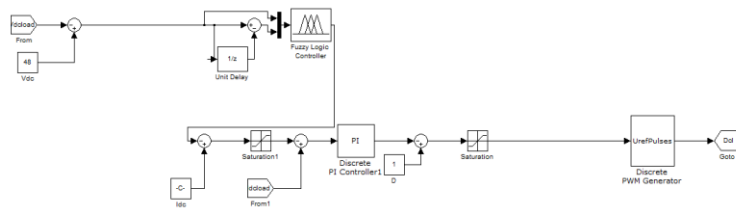
Fig 8. MATLAB/SIMULATION diagram of proposed wind and wave system
