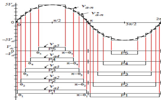
Fig.2 Output phase voltage waveform of an 11-level cascade inverter with 5 separate dc sources.
