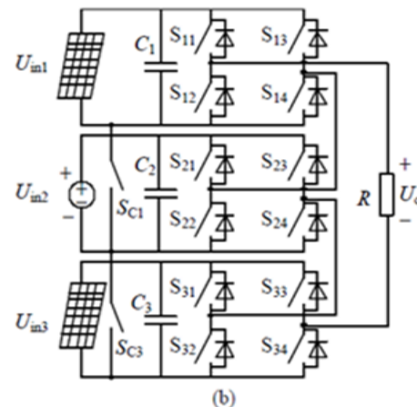
Topologies of the proposed inverter. (a) The novel single dc source cascaded seven-level inverter. (b) Three-input cascaded
