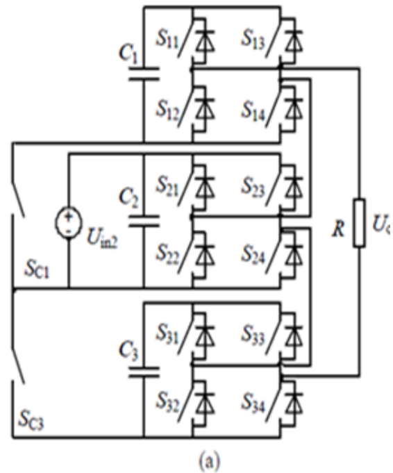
Topologies of the proposed inverter. (a) The novel single dc source cascaded seven-level inverter. (b) Three-input cascaded
