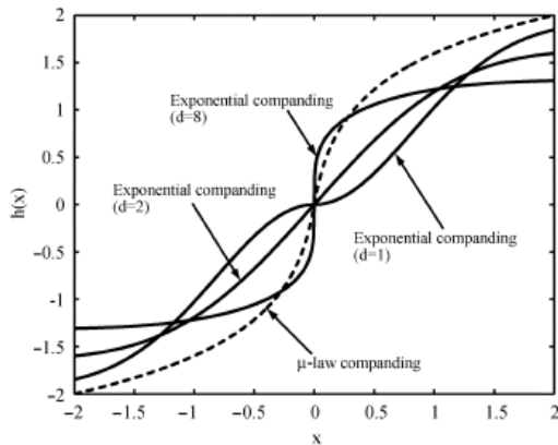
Fig. 2. The exponential commanding function h(x) .
