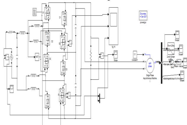
Fig.14 Simulink model of single-phase AC-AC converter with Induction Motor drive
