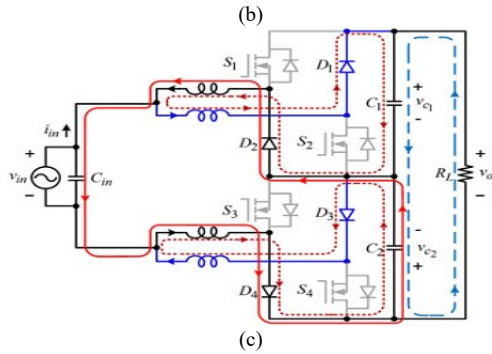
Fig.6. Operation of the proposed boost type ac-ac converter during dead time. (a) Dead time. (b) v_{in} > 0 . (c) v_{in} < 0 .
