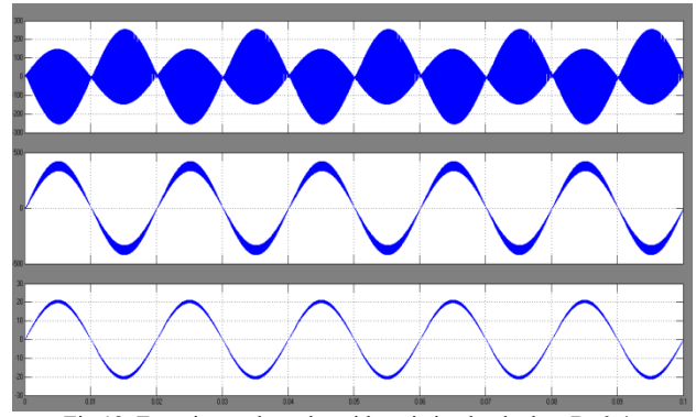
Fig.12. Experimental results with resistive load when D=0.4 . Waveforms of input inductor voltage, output voltage and input inductor current.
