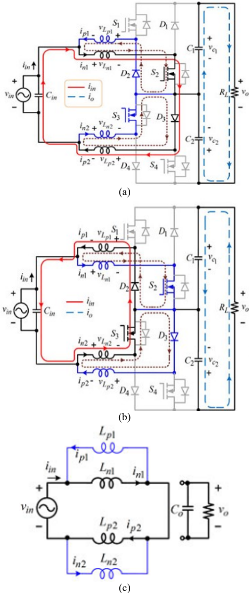
Fig.4. Mode 1 of the proposed boost-type ac-ac converter. (a) v_{in} > 0 . (b) v_{in} < 0 . (c) Simplified equivalent circuit of mode 1 for v_{in} > 0 .
