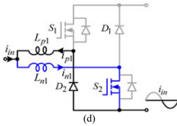
Fig.3. Conduction states of the proposed boost-type ac-ac converter. (a) i_{in} > 0 and S2 on. (b) i_{in} > 0 and S2 off. (c) i_{in} < 0 and S1 on. (d) i_{in} < 0 and S1 off.
