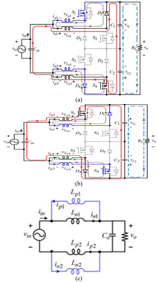
Fig.5. Mode 2 of the proposed boost type ac-ac converter. (a) v_{in} > 0 . (b) v_{in} < 0 . (c) Simplified equivalent circuit of mode 2 for v_{in} > 0 .
