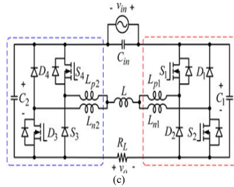
Fig.2. Proposed single-phase ac-ac converters. (a) Buck type. (b) Boost type. (c) Buck-boost type.
