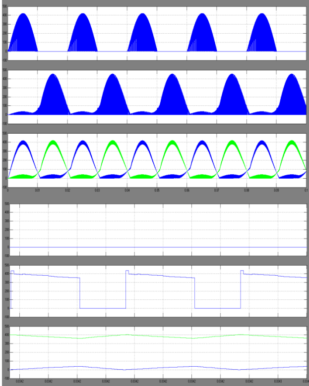
Fig.11 Experimental results with a resistive load when D=0.4 . (a) Waveforms of voltages across capacitors C1 and C2 and drain to source voltages of S2 and S4. (b) Magnification of waveforms in (a).
