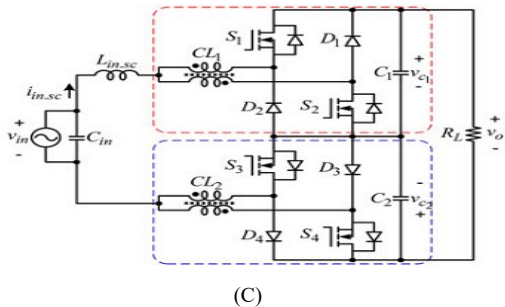
Fig.1. Boost-type dc-dc and ac-ac direct PWM converters. (a) Traditional dc-dc converter. (b) Traditional ac-ac converter. (c) SC ac-ac converter [13]
