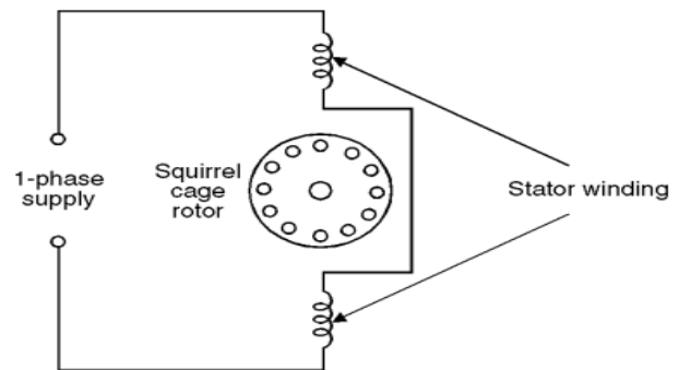
Fig.8 Single-phase induction motor
