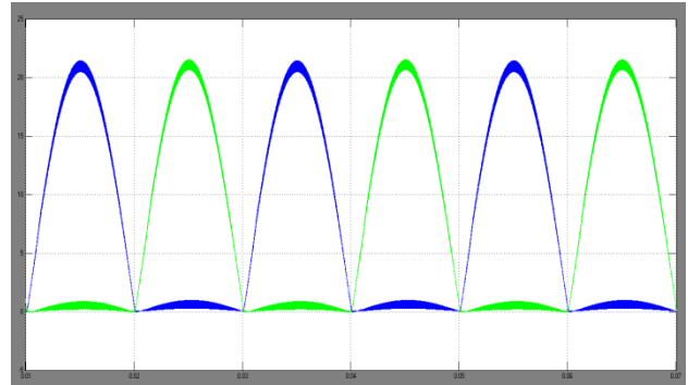
Fig.13. Experimental results with resistive load when D=0.4 . Current Wave forms of limiting inductors.
