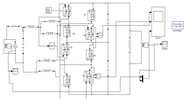
Fig.9 Simulink model of single-phase AC-AC converter
