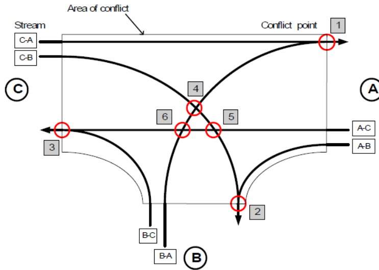
Fig 3.1: Scheme of Conflict of Traffic Streams
