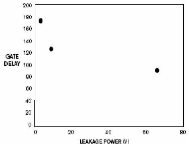
Figure4: Tradeoff between leakage and Power
