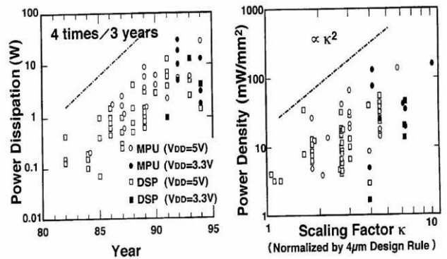
Figure 1: Evolution in Power dissipation [15]
