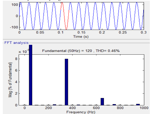
Fig.20.Total harmonic distortion for UPQC with fuzzy compensated system, THD=0.46%.
