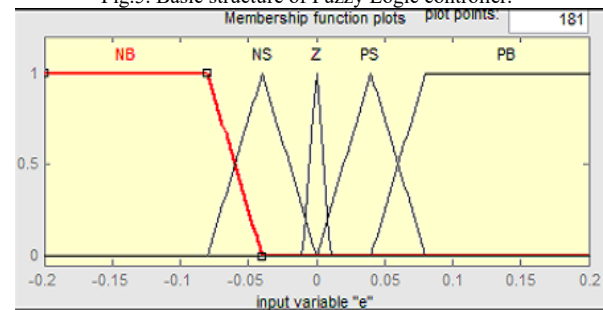
Fig.6. Error as input
