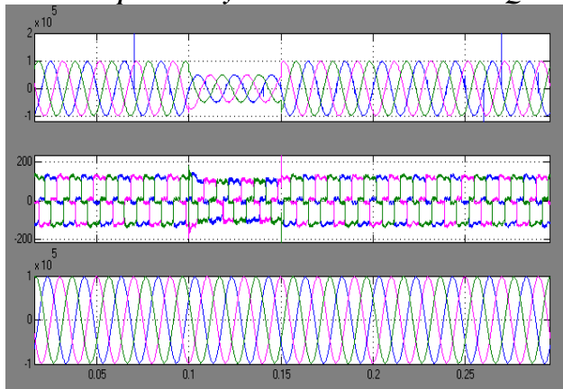
Fig.14. Supply voltage, Load current, load voltage for with UPQC on sag condition.
