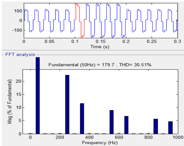
Fig13.Total harmonic distortion for uncompensated system, THD =30.51%
