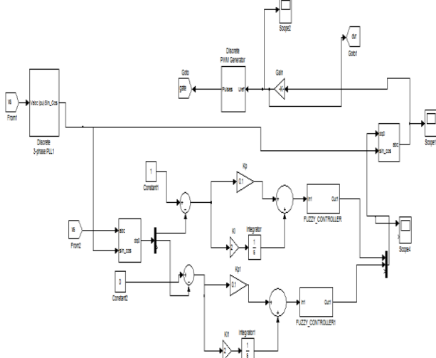
Fig.18.Hybrid Fuzzy logic control block diagram for UPQC system.
