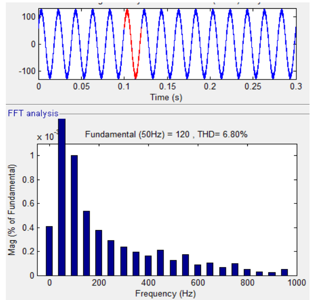
Fig.15.Total harmonic distortion for UPQC compensated system, Base THD =6.80%.
