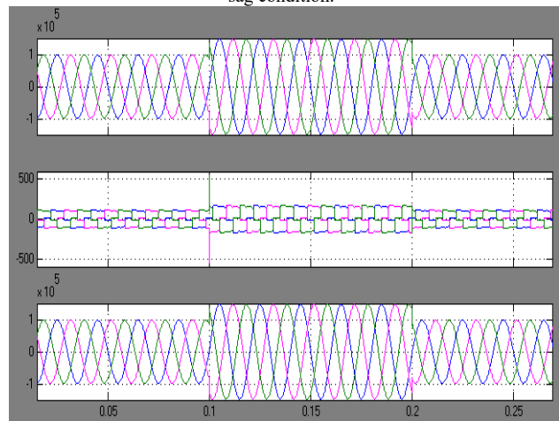
Fig.12. Supply voltage, Load current, load voltage for without UPQC on swell condition
