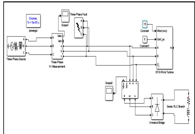
Fig.10. Matlab/Simulink circuit diagram for uncompensated system.
