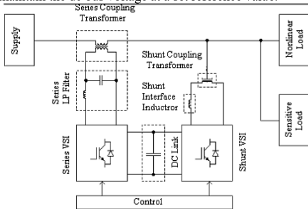
Fig.2. Schematic diagram of Unified Power Quality Conditioner.
