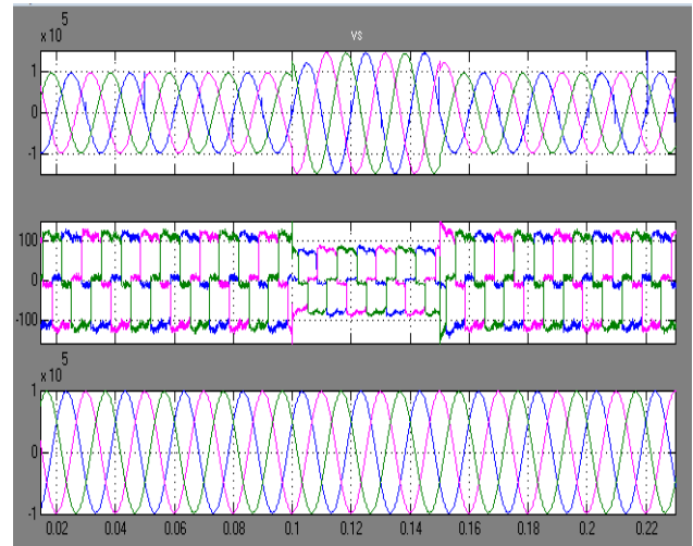
Fig.19.Supply voltage, Load current, load voltage for UPQC with Hybrid Fuzzy Logic Controller on Swell condition.
