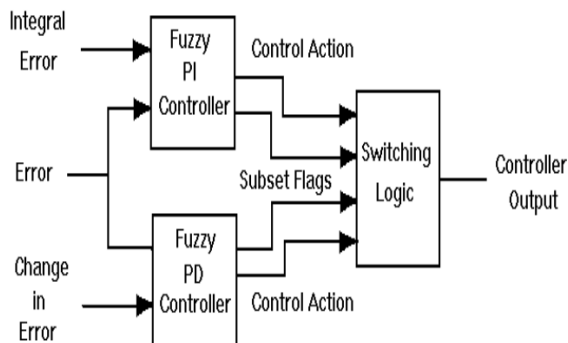
Figure.9. Hybrid Fuzzy PID Controller.
