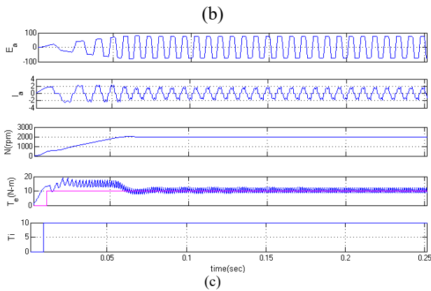
Fig.5 Starting and steady-state performances of the proposed SPV array-based zeta converter-fed BLDC motor drive for water pump. (a) SPV array variables. (b) Zeta converter variables. (c) BLDC motor-pump variables.
