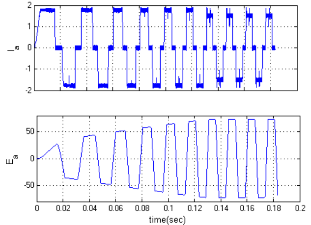
Fig.11 Stator current and emf.
