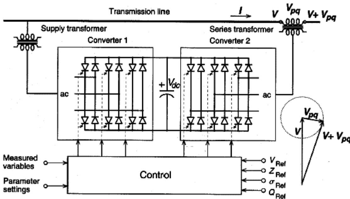
Fig – 3. Unified Power Flow Controller
