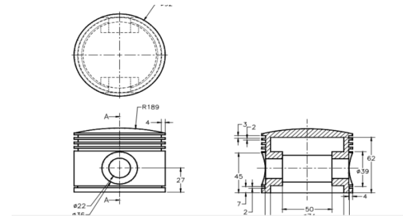
Dimensions for piston
