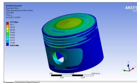
Deformation
