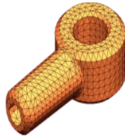
Model subdivided into small pieces (elements)
