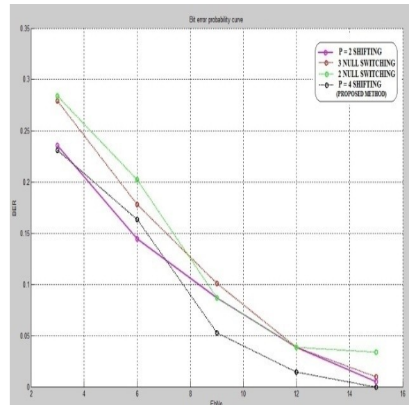
Figure 5.6 BER against SNR A_{\gamma} = 3 dB with p = 2 [25], switching by 3 & 2 null subcarrier and p = 4 .
