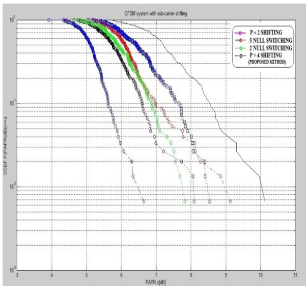
Figure 5.5 The PAPR's CCDF @ p = 2 [1], switching by 3 & 2 null subcarrier, null switching and p = 4 .
