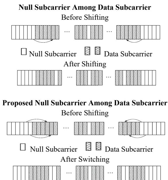
Figure 4.3 Shifting null subcarrier among data subcarrier and proposed shifting null subcarrier among data subcarrier
