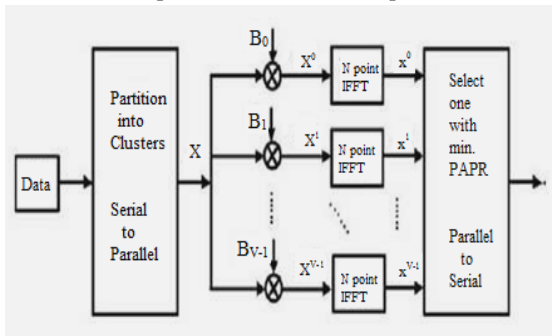
Figure 3.2 Block diagram of selected mapping method .
