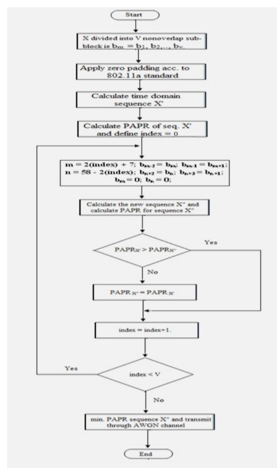
Figure 4.4 Flow chart for proposed method
