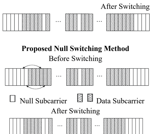
Figure 4.2 Comparison between null switching method and proposed null switching method
