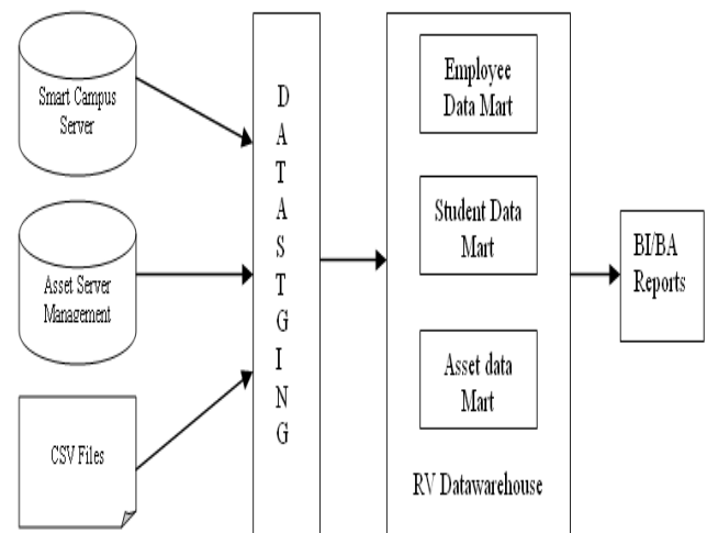
Fig. 1. Engg_Data warehouse architecture
