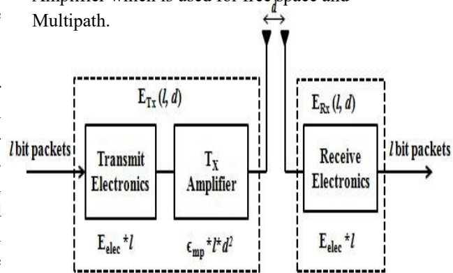
Figure 2: Radio Model
