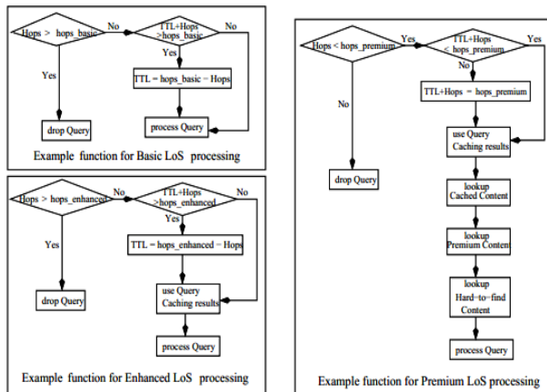
Figure3: Functions for service differentiation during content search.
