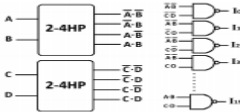
Fig: 4-16HPI line decoder
