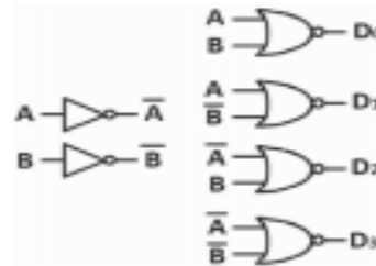
Fig: Non-inverting NOR-based decoder
