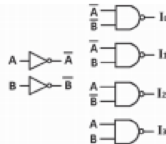
Fig: Inverting NAND-based decoder
