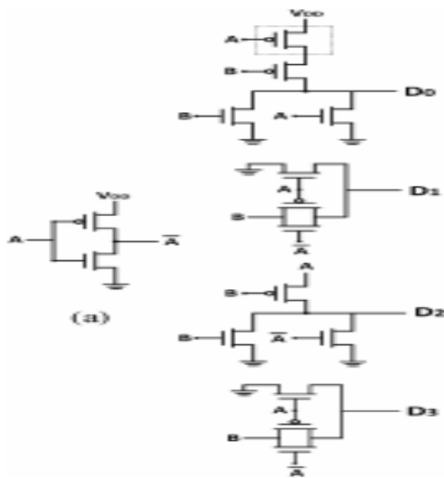
Fig: New 14-transistor 2-4 line decoders
