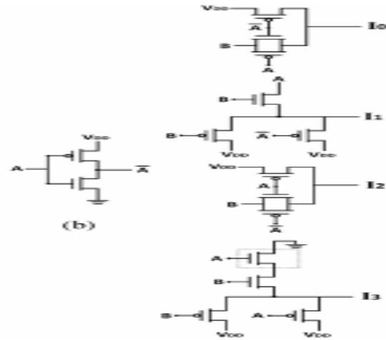
Fig: New 15-transistor 2-4 line decoders
