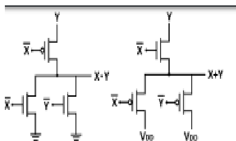
Fig: AND/OR gates using DVL
