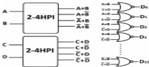
Fig: 4-16HP line decoder
