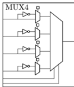
Fig 2: MUX4 LE depicting optional data input inversions
