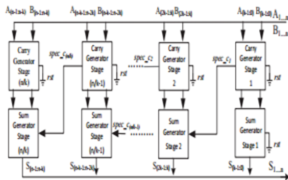
Fig1: Circuit Scheme of ETAII.
