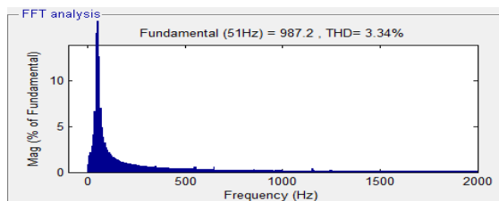
Fig.14. FFT Analysis
