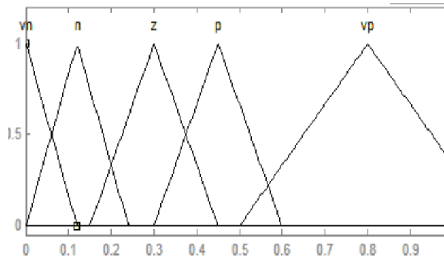
Fig.7. membership function representation for input 1
