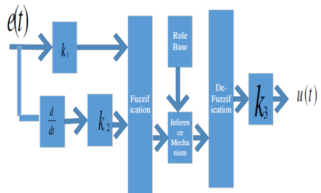
Fig.6. Block diagram of Fuzzy Logic Controller
