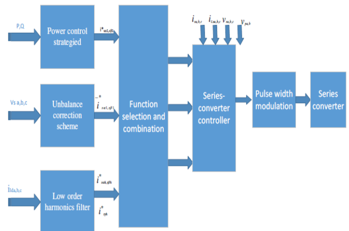
Fig.3.Control Diagram of series converter
