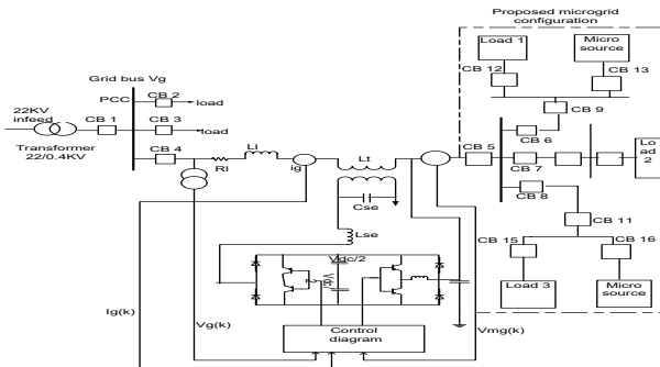
Fig.1. Configuration of Proposed FACTS device based Microgrid system
