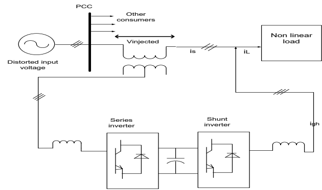
Fig.2.structure of unified power quality conditioner
