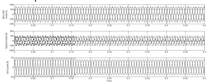
Fig.11. Simulation result for Grid, Series Converter and Micro-Grid Voltage
