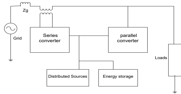
Fig.5. Configuration of UPQC system with DG
