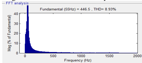
Fig.13. FFT Analysis Case 2: with fuzzy controller:
