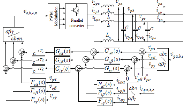
Fig.4. Control Diagram of shunt converter
