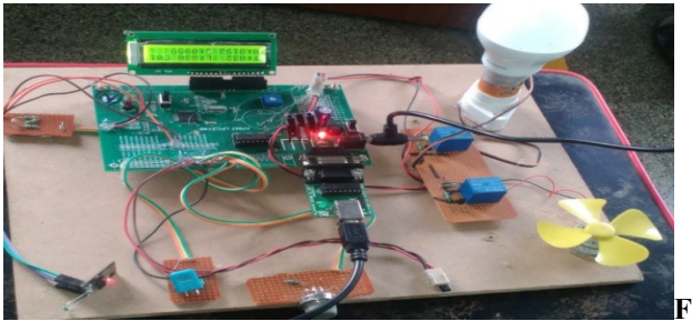
Fig 5 Kit prototype of sensor node-1 working condition 6.2 SENSOR NODE-2
