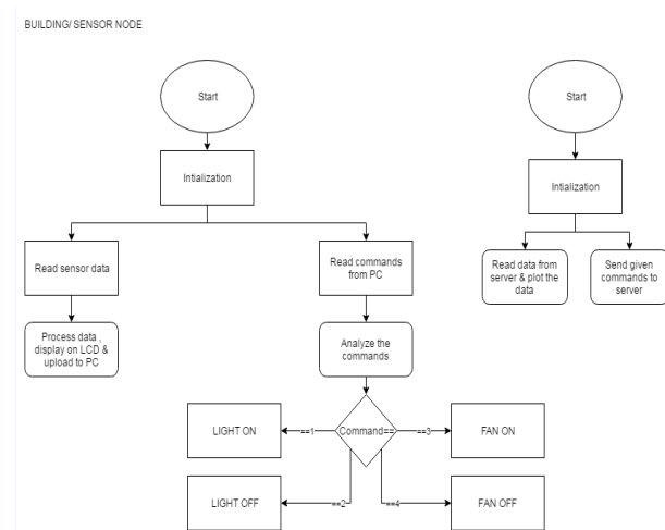
Fig 3 Flow Diagram of building/sensor node
