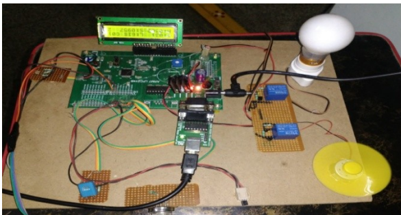
Fig 7 Kit prototype of sensor node-2 giving toggle to the bulb when command=3
