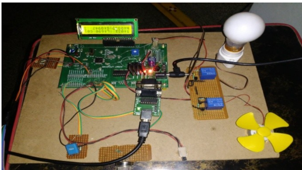
Fig 7 Kit prototype of sensor node-2 giving toggle to the bulb when command=3
