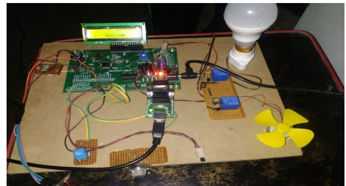
Fig 4 Kit prototype of sensor node-1
