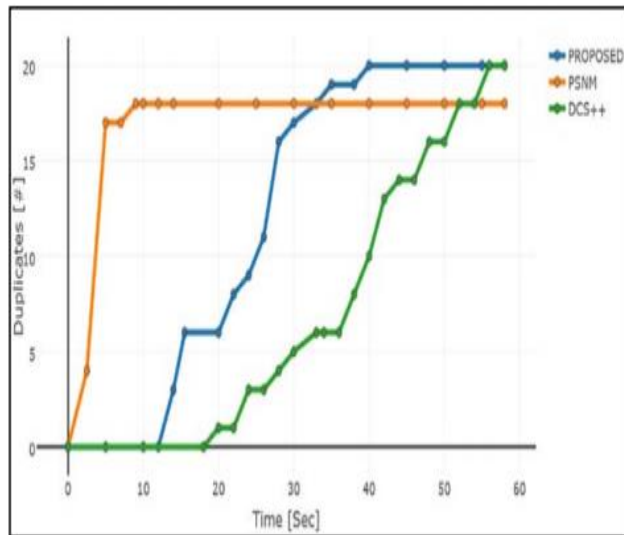
Fig 3: Comparison of duplicates found by psnm
