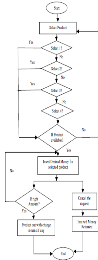
Figure 3: Flow Chart for Proposed Vending Machine
