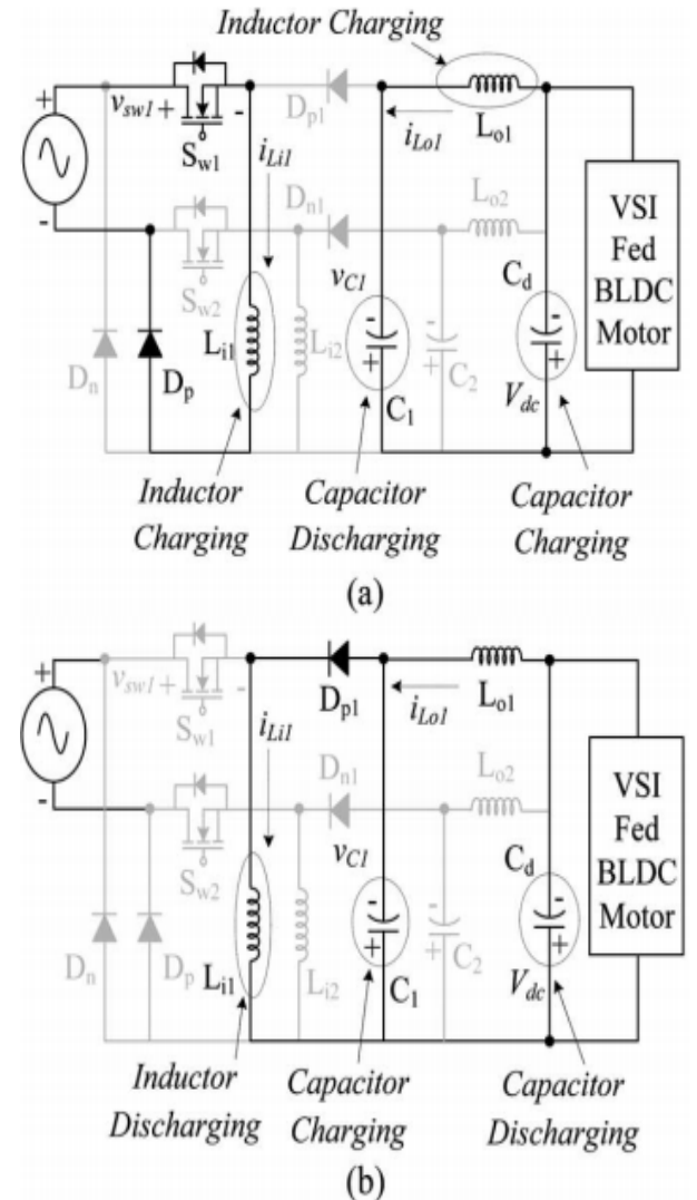
Fig. 2. Proposed PFC BL-Luo converter-fed BLDC motor drive.
