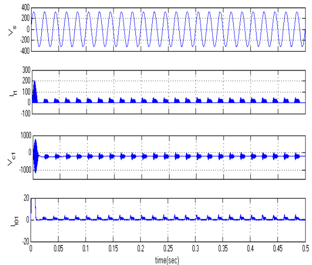
Fig.10. Simulink results of V_s , I_{i1} , V_{c1} & I_{i01} .
