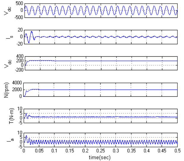
Fig.13. Simulink results of proposed BLDC motor drive showing dynamic performance of the during change in supply voltage from 250 to 180
