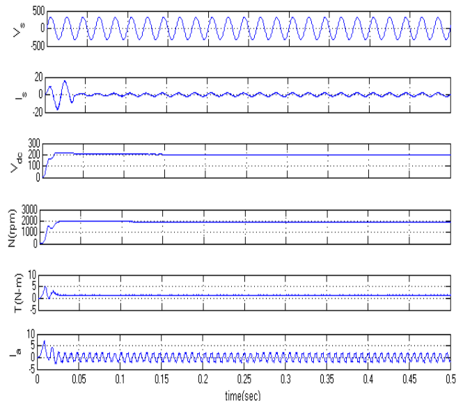
Fig.8. Simulink results of proposed BLDC motor drive At rated load torque on BLDC motor with V_{dc} = 200 V and V_s = 220 V.
