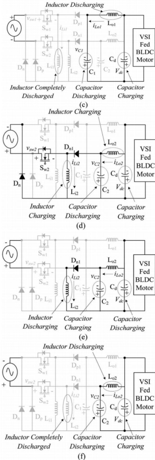
Fig. 3. Different modes of operation of the PFC BL-Luo converter during (a-c) positive and (d-f) negative half cycles of supply voltage.
