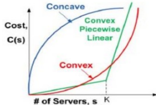
Fig 2. Cost Functions
