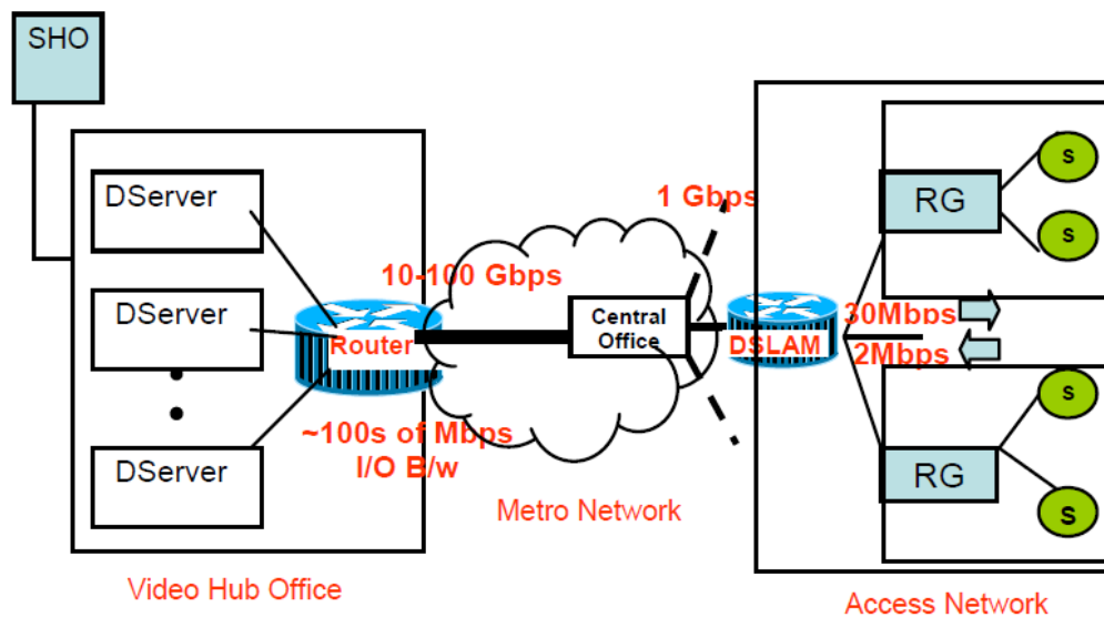
Fig. 2 IPTV Architecture
