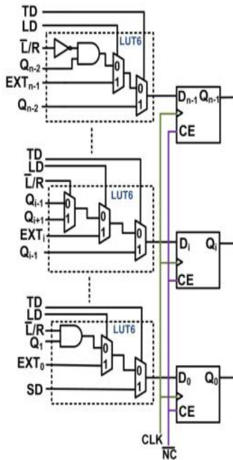
Fig. 5. Proposed architecture for scan FF inserted universal shift register and n FFs.
