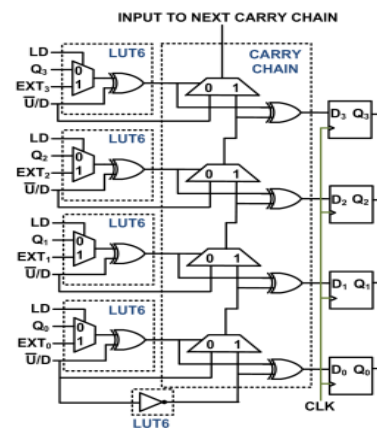
Fig. 2. Original architecture for loadable bidirectional counter.
