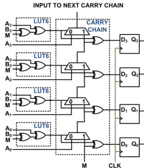
Fig. 7. Original pipelined adder subtractor design.
