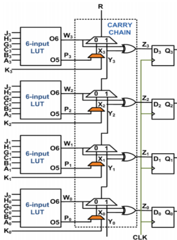
Fig. 1. A simplified Virtex-7 slice architecture.
