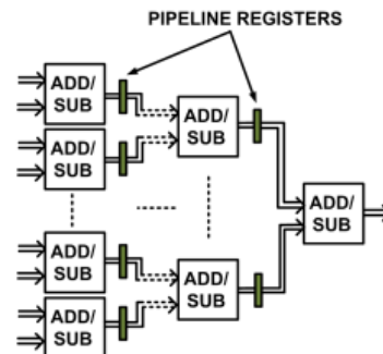
Fig. 6. Block diagram of pipelined adder subtractor tree.
