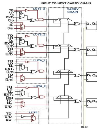
Fig. 3. Proposed architecture for scan FF inserted loadable bidirectional counter. (The added functionality of the LUTs is shown in brown.)
