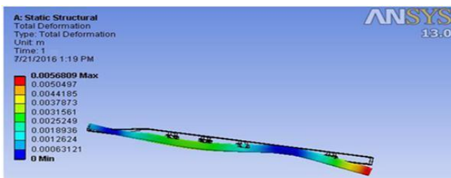
Fig 7: Total deformation in frame (Structural steel)
