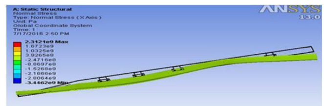
Fig 8: Normal Stress Distribution in Frame (S-glass/ Epoxy)
