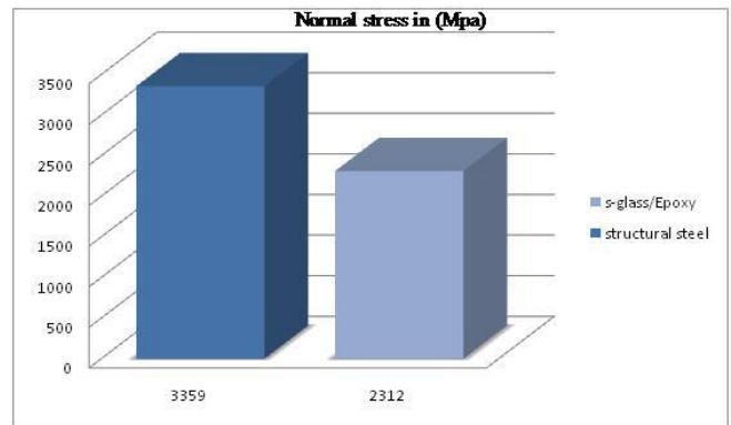
Fig 13: Graphical representation of Normal stress
