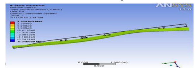
Fig 5: Normal Stress Distribution in Frame (Structural Steel)
