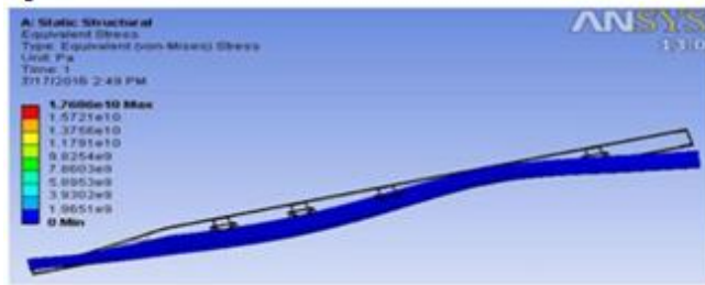
Fig 6: Equivalent Stress Distribution in Frame (Structural Steel)
