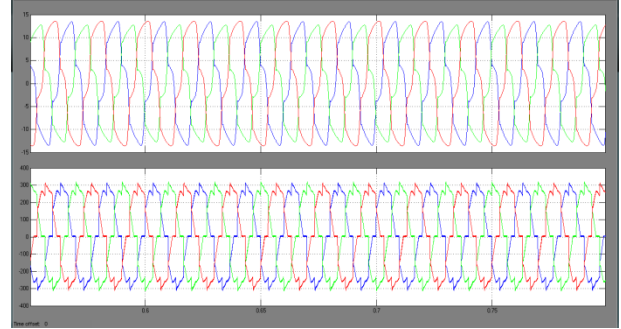
(a) Simulation waveform for IabcT, VabcT without D-STATCOM
