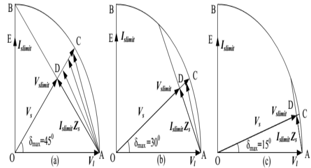
Fig.3. Voltage regulation performance curve of DSTATCOM at different R_s/X_s . (a) For R_s/X_s = 1 . (b) For R_s/X_s = \sqrt{3} . (c) For R_s/X_s = 3.73 .
