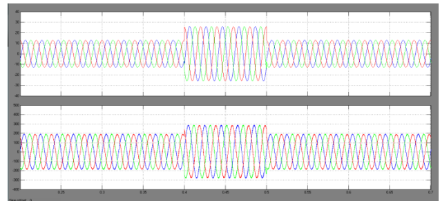
(a) Simulation waveform for Proposed D-statcom of IabcT, voltage swell VabcT
