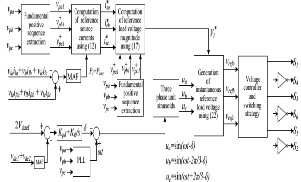
Fig.6. Block diagram of proposed flexible control strategy.
