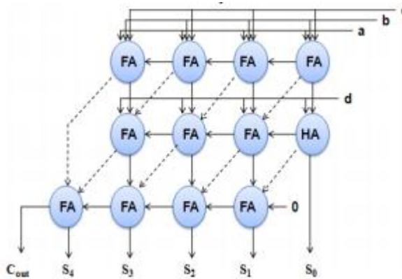
Fig. 6: Carry Save Adder
