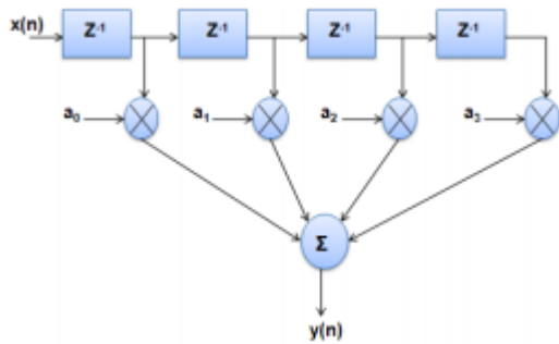
Fig. 1: FIR Filter
