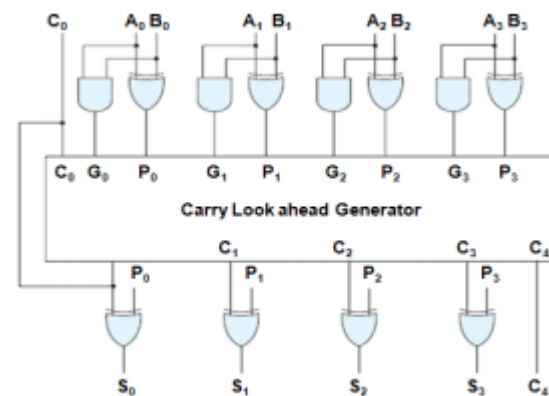
Fig. 4: Carry Look Ahead Adder
