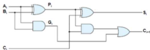
Fig. 3: Carry Look Ahead Generator
