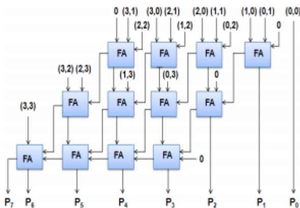
Fig. 7: Array Multiplier
