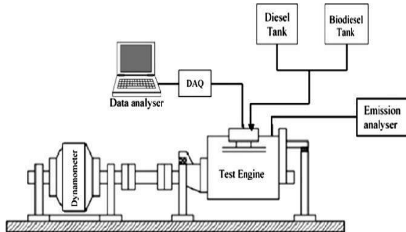
Figure2. Experimental setup (Jalpit B. Prajapati, et al., 2014)
