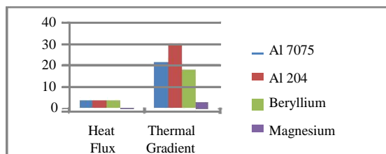
Figure 38: Results of Thermal Gradient and Heat Flux of All Materials With Curve Shape and Thickness of 2.5 mm
