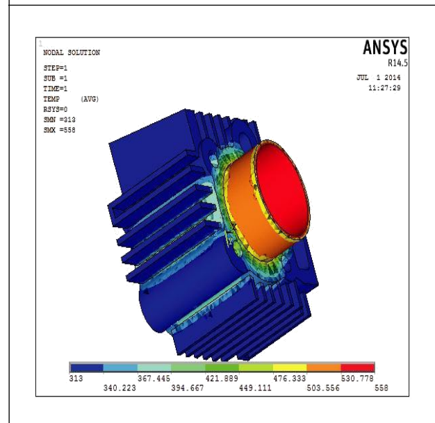
Figure 15: Rectangle Shaped Beryllium at Nodal Temperature With 3mm Thickness
