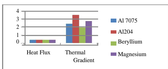
Figure 41: Results of Thermal Gradient and Heat Flux of All Materials With Curve Shape and Thickness of 3 mm
