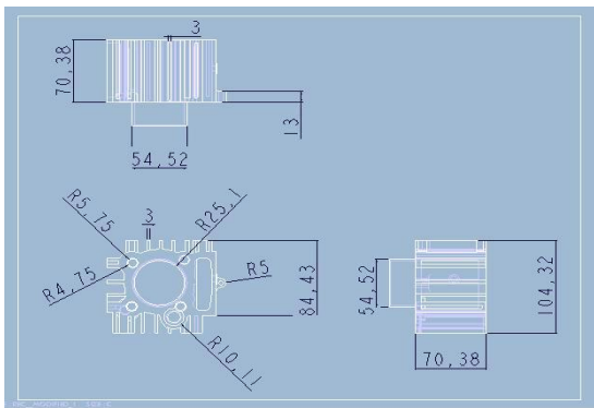
Figure 5: Rectangular Shape FIN Body With 3mm Size
