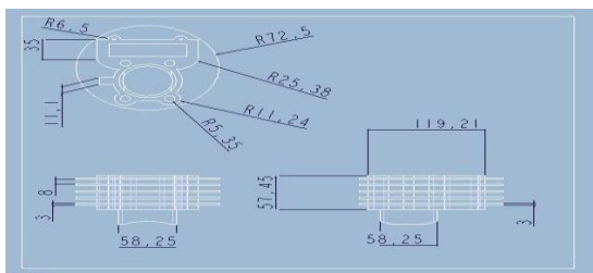
Figure 6: Circular Shape FIN Body With 3mm Size
