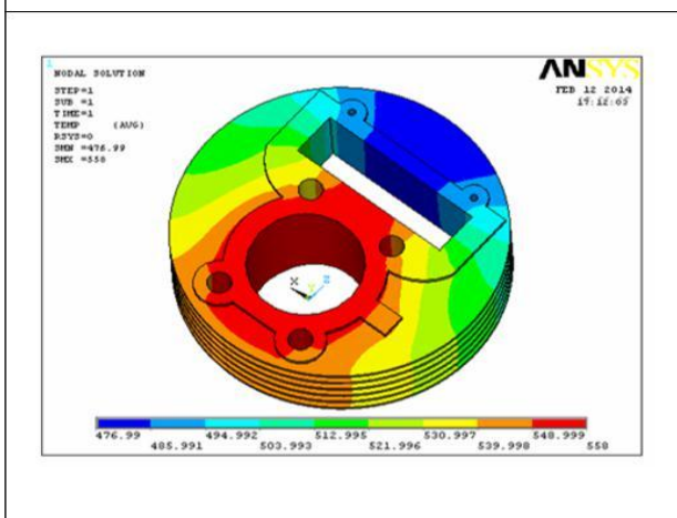
Figure 25: Circular Shaped Aluminum Alloy 204 at Nodal Temperature With 2.5mm Thickness
