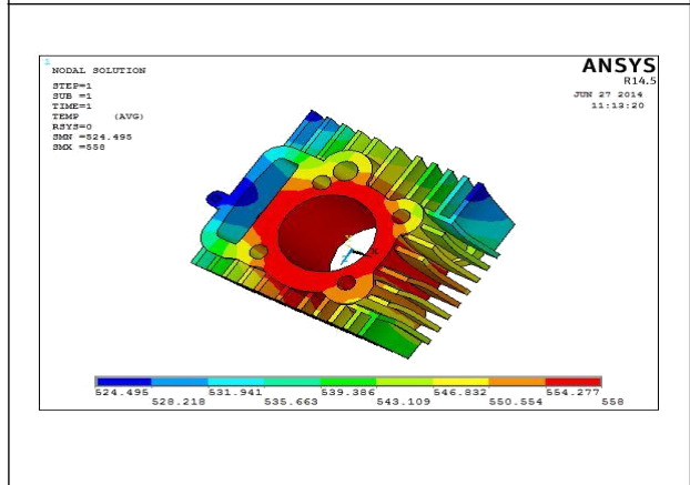
Figure 32: Curve Shaped Aluminum Alloy 7075 at Nodal Temperature With 3mm Thickness
