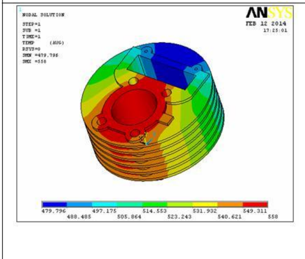
Figure 21: Circular Shaped Aluminum Alloy 204 at Nodal Temperature With 3mm Thickness
