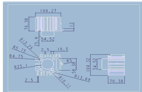
Figure 8: Rectangular Shape FIN Body With 2.5mm Size
