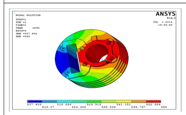
Figure 27: Circular shaped Aluminum Alloy 7075 at Nodal Temperature With 2.5mm t
