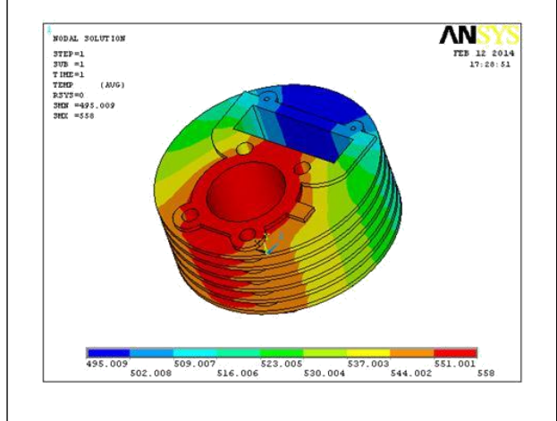
Figure 22: Circular Shaped Magnesium at Nodal Temperature With 3mm Thickness
