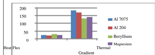
Figure 40: Results of Thermal Gradient and Heat Flux of All Materials With Rectangle Shape and Thickness of 2.5 mm
