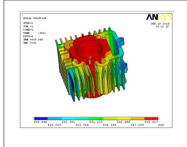
Figure 34: Curve Shaped Aluminum Alloy 204 at Nodal Temperature With 2.5mm Thickness
