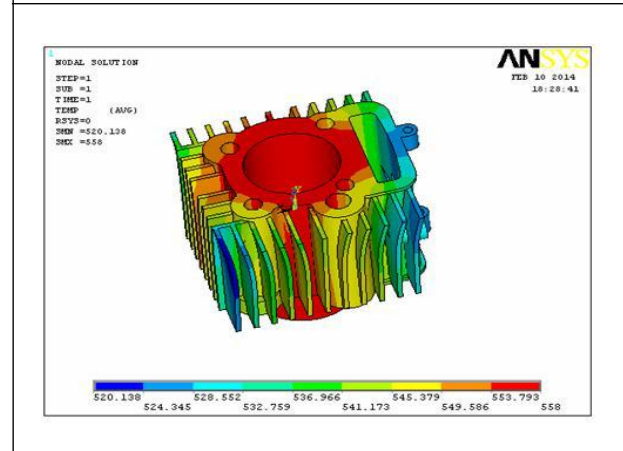
Figure 35: Curve Shaped Magnesium at Nodal Temperature With 2.5mm Thickness
