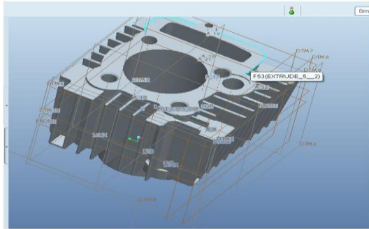
Figure 4: Original Fin Body
