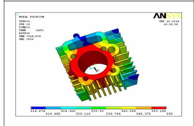
Figure 30: Curve Shaped Aluminum Alloy 204 at Nodal Temperature With 3mm Thickness
