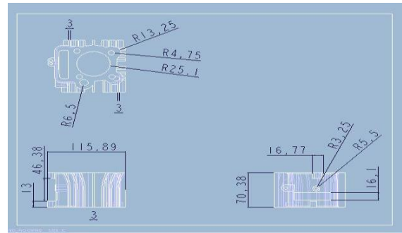
Figure 7: Curve Shape FIN Body With 3mm size
