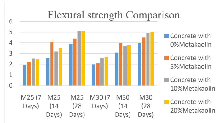
Fig. 8.42: Comparison of Flexural strength of Conventional Concrete and Concrete with Metakaolin
