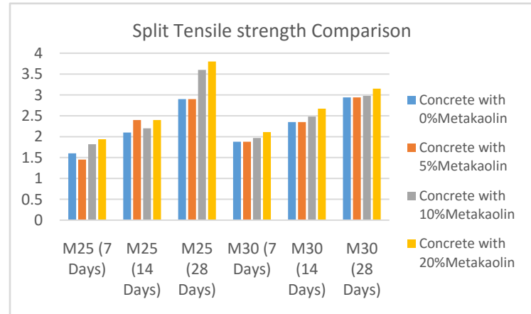
Fig. 8.2: Comparison of Split Tensile strength of Conventional Concrete and Concrete with Metakaolin
